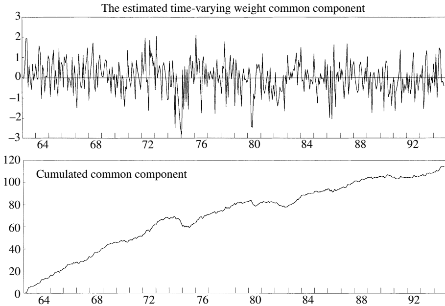
Fig. 3. The Estimated Time-varying Weight Common Component
